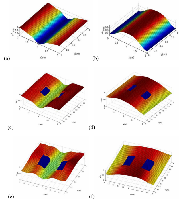
Fig. 7 Time-average plots of MinD and MinE dynamics from the LBM with and without obstacles. The MinD protein is shown in terms of the time-averaged density for the obstacles 0,4,9 percents of cell size as shown in (a), (c), (e), respectively. The MinE protein is shown in terms of time-averaged density for the obstacles 0,4,9 percents of cell size as shown in (b), (d), (f), respectively
